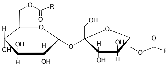
Figure 1 – Sucroglyceride molecule
